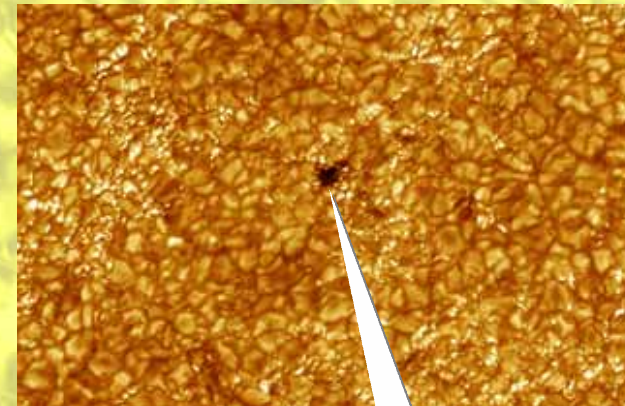
Pore
