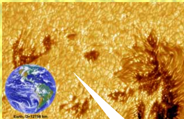
Granulation
