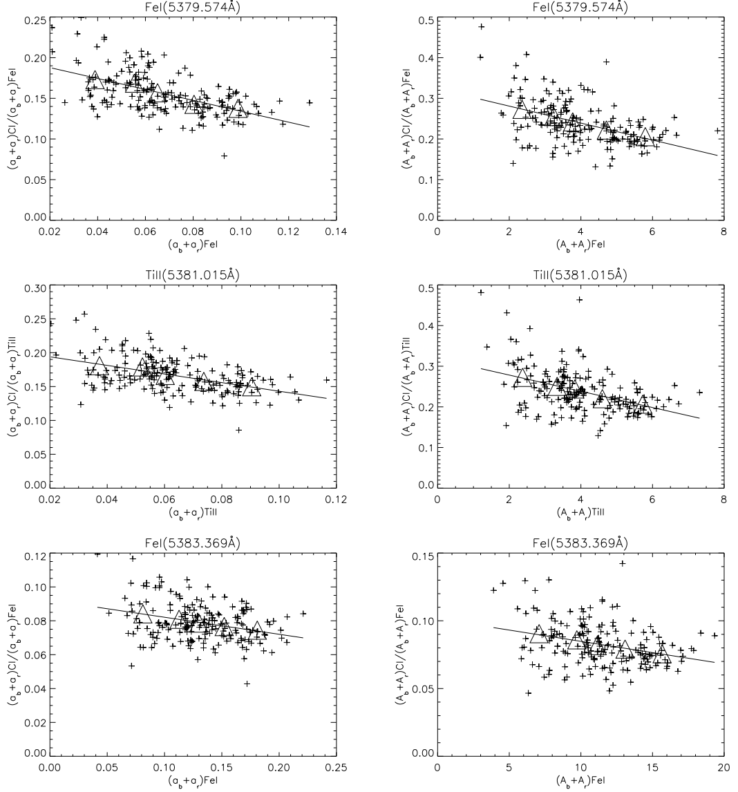
Figure 3. Stokes V amplitude (left) and area (right) ratios of C I (5380.3 Å) to Fe I 5379.6 Å (top), Ti II 5381.0 Å (middle) and Fe I 5383.4 Å (bottom). A_b : area of Stokes V/I blue wing, A_r : area of the Stokes V/I red wing, a_b : amplitude of the Stokes V/I blue wing, a_r : amplitude of the Stokes V/I red wing. The line shows the linear fit to the data points. Triangles represent 37 point averages.
