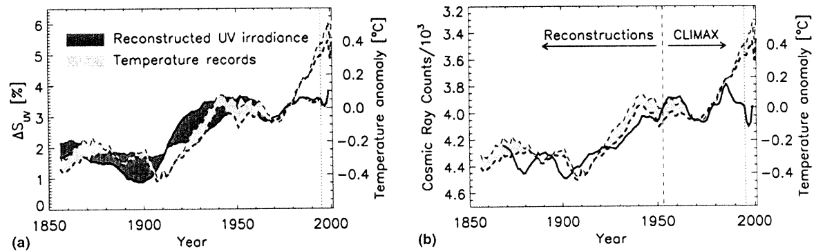
Fig. 2. (a) The same as Fig 1(a), but for UV irradiance (solid curves). From 1986 onwards Mg II measurements are shown (solid and dot-dashed lines represent compilations by Viereck and Puga, 1999 and Cebula et al., 1992, respectively). (b) The same as Fig. 1, but now exhibiting a composite of cosmic ray flux (solid) instead of irradiance.
