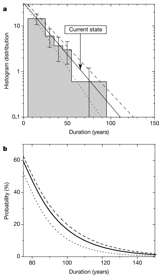
Figure 4 Distribution of the duration of episodes of high solar activity and the probability that the current episode will reach a given duration. a , Histogram of the distribution function of the duration of episodes of high solar activity during which the 10-year averaged SN exceeds 50. Some bins have been enlarged in order to improve the statistics; in such cases the average number per bin is given. The vertical error bars correspond to \sqrt{N} , where N is the number of events combined in one data point. The length of the current period of high activity is marked by the arrow. The solid line is a least-squares exponential fit to the plotted points. The dashed and dotted lines represent exponential fits to the distributions obtained from extreme SN reconstructions including the influence of random and systematic errors as given in Fig. 3 (see also the discussion in Supplementary Information). b , The probability of the total duration of a state of high activity (SN level exceeding 50). For the current episode, which started in AD 1940 (~ 65 years ago), the start of the diagram corresponds to the year AD 2015. Each curve is based upon the corresponding fit shown in a . The probability (for the reference curve) that the high activity continues for another 5 decades for a total duration of 115 years is only 8%.
