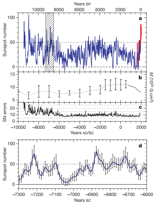
Figure 3 Reconstructed sunspot number and its uncertainty for the whole interval of time considered. a , 10-year averaged SN reconstructed from Δ 14 C data since 9500 bc (blue curve) and 10-year averaged group sunspot number 1 (GSN) obtained from telescopic observations since 1610 (red curve). The horizontal dotted line marks the threshold above which we consider the Sun to be exceptionally active. It corresponds to 1.3 standard deviations above the mean. b , Evolution of the virtual geomagnetic dipole moment 26 with error bars that take into account the scatter between different palaeomagnetic reconstructions. (The error bars give the s.d. in the reconstructed virtual geomagnetic dipole moment.) The geomagnetic field data of ref. 25 are given by the dotted line. c , Uncertainty in the reconstructed SN. It includes errors introduced at each step of the reconstruction process. The largest sources of random errors are the uncertainty in the knowledge of the geomagnetic dipole moment and in the 14 C production rate. We also consider systematic errors—for example, due to uncertainties in the 14 C production rate prior to the considered period of time. A discussion of how these uncertainties are estimated is given in Supplementary Information. Clearly, the uncertainties are sufficiently small that they do not affect the presence or absence of grand minima or of episodes of high activity, except in already marginal cases. d , A detail from the full time series of reconstructed SN with expanded temporal scale. The chosen interval (corresponding to the shaded part of a ) exhibits three episodes of high solar activity and a grand minimum. The error bars indicate the total uncertainty, \sigma , in the reconstruction. (They depict the 68% confidence interval for the reconstructed SN, which takes into account both random and systematic uncertainties (see Supplementary Information).) The two strongest maxima lie 2.1 \sigma and 3.0 \sigma , respectively, above the high-activity threshold of 50. Hence the probability that they are due to statistical fluctuations related to these errors is 3% and 0.2%, respectively. The probability that a whole episode of high activity (lasting, say, 50 years) is due to a statistical fluctuation is significantly smaller.
