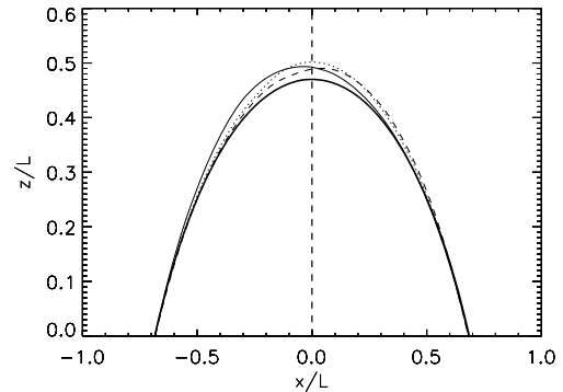
Fig. 7. MHD simulations of swaying-like loop oscillations excited by a hot pulse launched at (x_0/L, z_0/L) = (-0.42, 0) where L = 100 \text{ Mm} (for details see Selwa et al. 2006 ). The curves indicate the positions of a field line in the oscillating loop at a series of times: t = 0 (thick solid line), t = 200 \text{ s} (thin solid line), t = 300 \text{ s} (dotted line), and t = 375 \text{ s} (dashed line).
