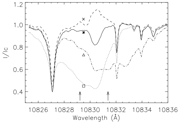
Fig. 2. Observed Stokes I profiles at different locations, indicated by the different symbols in Fig. 1b. Solid line (star symbol): quiet Sun profile. Dashed line (cross): He I emission profile. Dash-dotted line (triangle): very broad He I profile indicating multiple redshifted atmospheric components. Dotted line (square): deep absorption in the He lines, that is in part strongly blueshifted. The arrows mark the wavelengths at which images are shown in Fig. 4.
