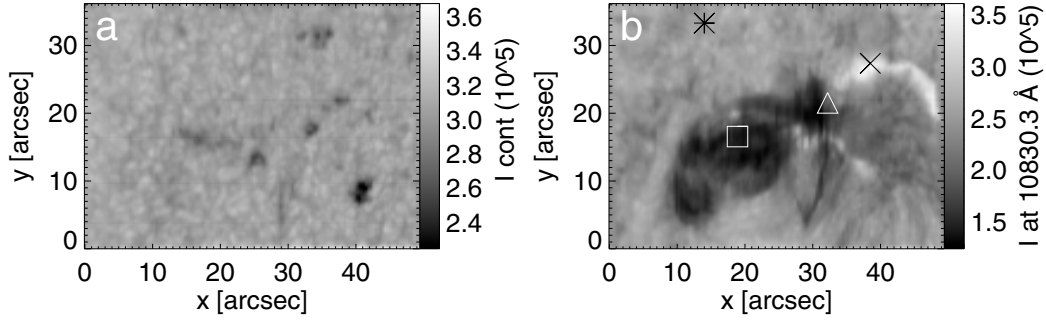
Fig. 1. Intensity maps at different wavelengths of the scanned portion of active region NOAA 10763 ( 24^\circ W, 14^\circ S). Left a): continuum. Right b): He I line core of the Tr2,3 component. The four symbols overlotted on the right image refer to the line profiles shown in Fig. 2.
