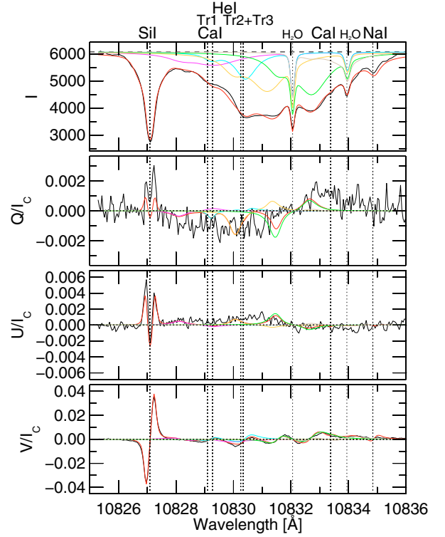
Fig. 12. Observed and inverted Stokes I , Q , U , and V profiles at the location ( 32'' , 21'' ) of the map in Fig. 1. The solid black lines are the observed profiles, while the red lines are the fits involving five different atmospheric components to describe the He I lines (magenta, light blue, yellow, green, and dark gray lines).
