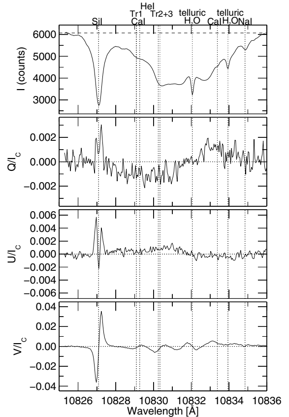
Fig. 3. Example of an observed averaged Stokes vector (dash-dotted profile of Fig. 2). The unusually broad Stokes I profile and the corresponding signatures of the V profile suggest that the He triplet samples multiple atmospheric components. The vertical dotted lines mark the rest wavelengths of the different lines that are present in the observed wavelength range and are identified at the top of the figure and listed in Table 1.
