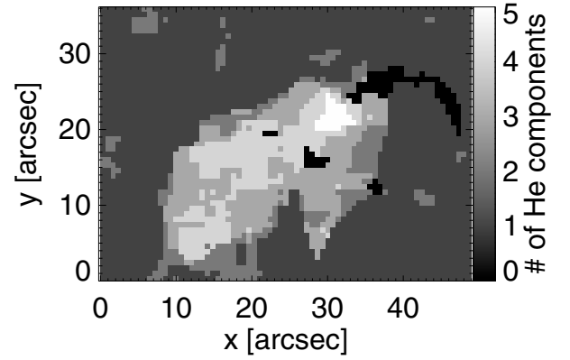
Fig. 6. Number of He components needed to fit the observed profiles for each pixel of the map. In the map, the pixels containing profiles that were not inverted are black (mainly those in which the He profile is in emission).
