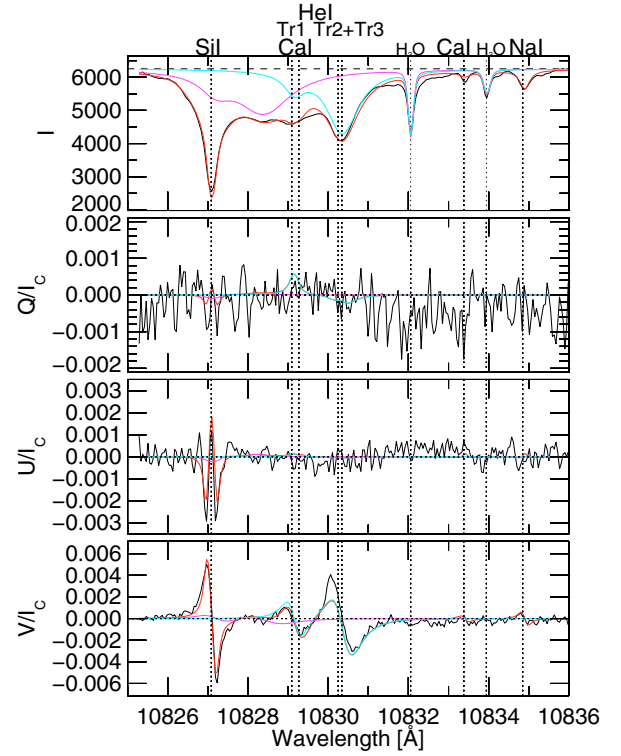
Fig. 9. Observed and inverted Stokes I , Q , U , and V profiles at the location ( 27'' , 9'' ) of the map in Fig. 1. The solid black lines are the observed profiles, while the red lines are the fits obtained imposing two different atmospheric components to describe the He I lines (the profiles of the individual components are given by magenta and light blue lines).
