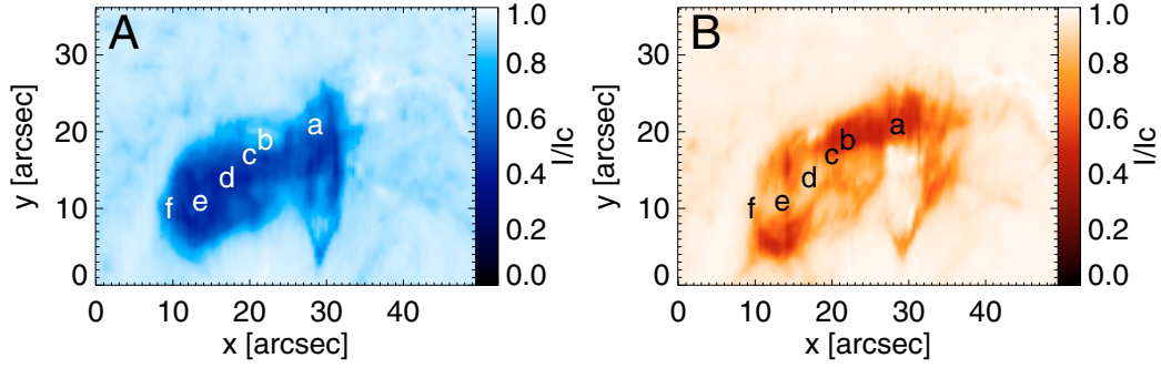
Fig. 4. Intensity maps of the scanned active region obtained at different wavelength positions indicated by arrows in Fig. 2. Left A ): At -30 \text{ km s}^{-1} with respect to the central rest position of the Tr2,3 component of the He triplet. Right B ): at +30 \text{ km s}^{-1} with respect to the central rest position of the Tr2,3 component of the He triplet. The different letters refer to the line profiles shown in Fig. 5.
