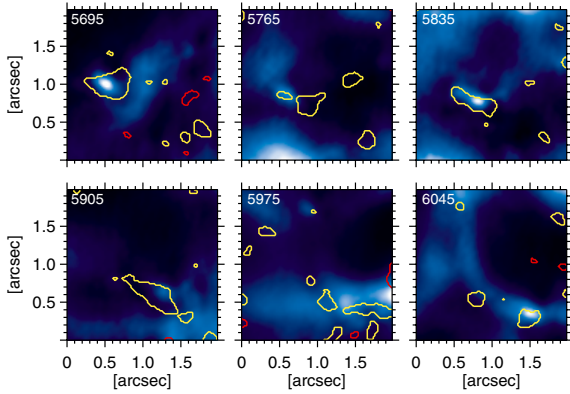
Fig. 7. Temporal evolution of a BP similar to the persistent flasher of Brandt et al. (1992). Time proceeds row by row from left to right in each row. The yellow and red contours indicate magnetic patches of opposite polarities. The time in seconds, from UT midnight, is given in the upper-left corner of each frame.
