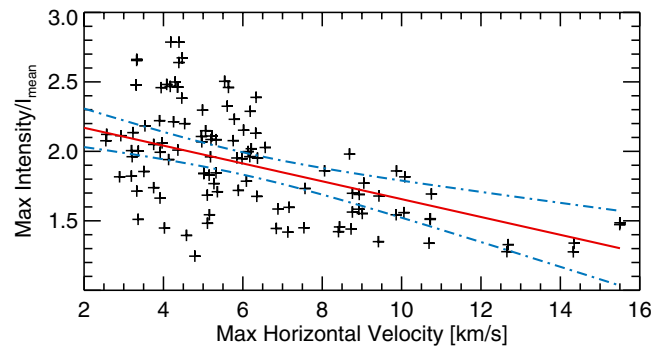
Fig. 12. Relationship between the maximum horizontal velocity and the maximum intensity of the identified BPs. The solid (red) line illustrates a linear regression fit to the data with 95% confidence bands (blue dot-dashed lines) around it.
