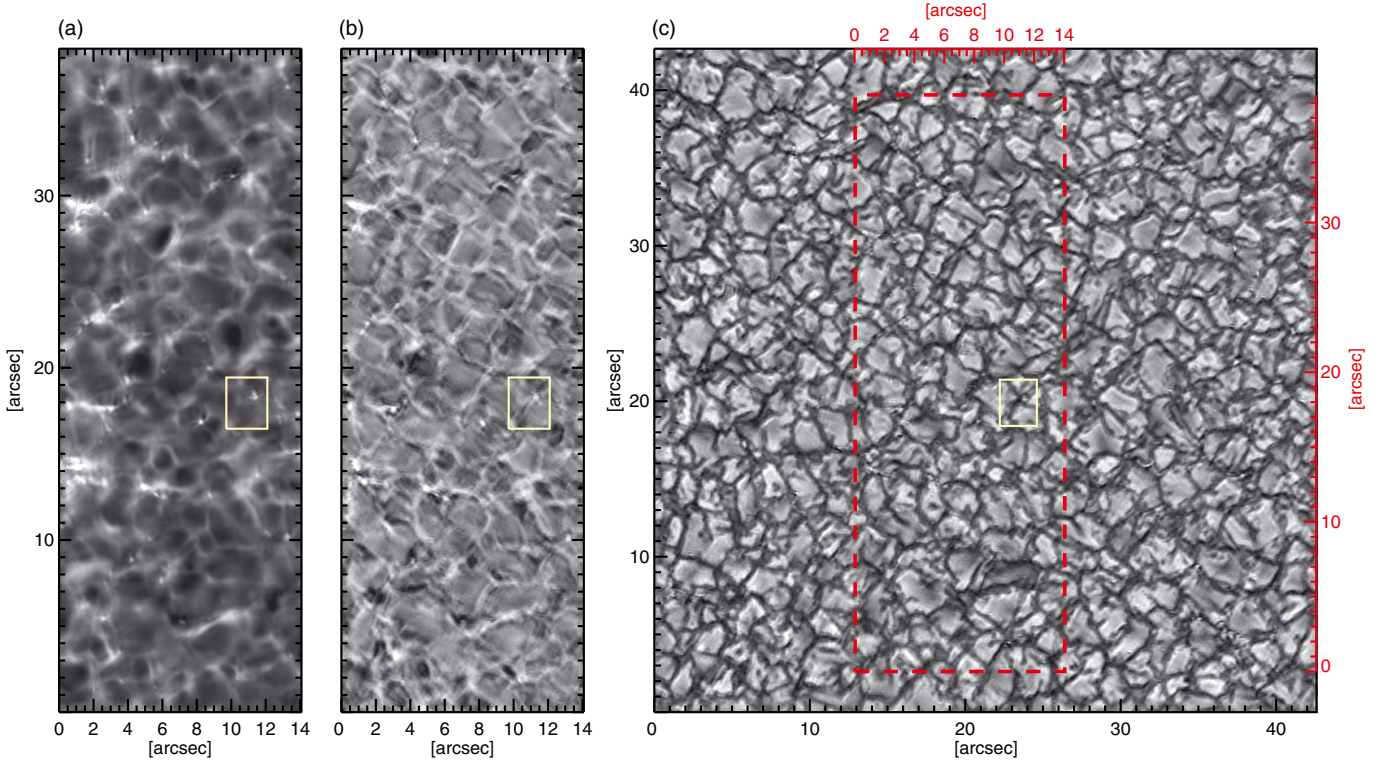
Fig. 1. Example of co-spatial and co-temporal images from both SuFI and IMAx instruments on board the SUNRISE balloon-borne solar telescope. a) SuFI Ca II H image. b) Average of two line-positions at -40 mÅ and +40 mÅ from the Fe I 5250.2 Å line-core. Plotted is the part of the full FOV overlapping with the SuFI Ca II H image. c) Full field of view of the continuum position of the IMAx Fe I 5250.2 Å line. The red dashed-line in this image illustrates the co-aligned area in common with the SuFI Ca II H image. The yellow box (solid-line) includes a sample Ca II H BP studied here; its temporal evolution and parameter fluctuations are presented in Figs. 4 and 5, respectively. The common coordinate system adopted for the present analysis is given below and to the left of panels a and b , as well as above and to the right of panel c .
