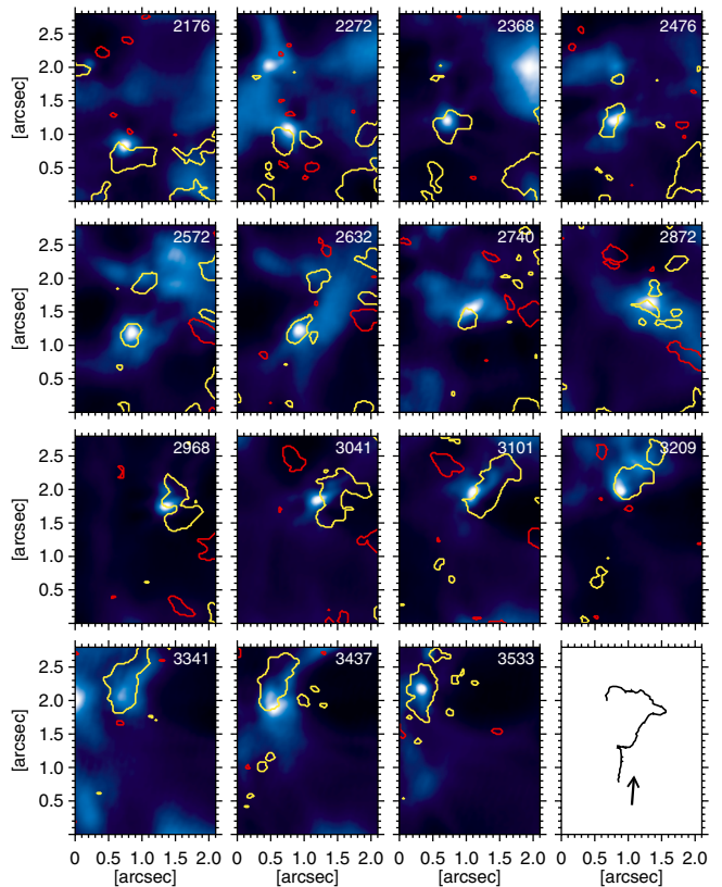
Fig. 4. Temporal evolution of a selected BP (Lifetime: 1321 s), observed on 9 June 2009 in the SUNRISE/SuFI Ca II H passband. Time proceeds row by row and from left to right within each row. The red and yellow contours outline magnetic regions with opposite polarities of the line-of-sight magnetic field component and match the 3\sigma level in Stokes V . In the bottom-right panel, the trajectory of the BP is plotted. The arrow marks the sense of the motion. The time from UT midnight, in seconds, is shown in the upper-right corner of each frame. Note the irregular intervals between frames.
