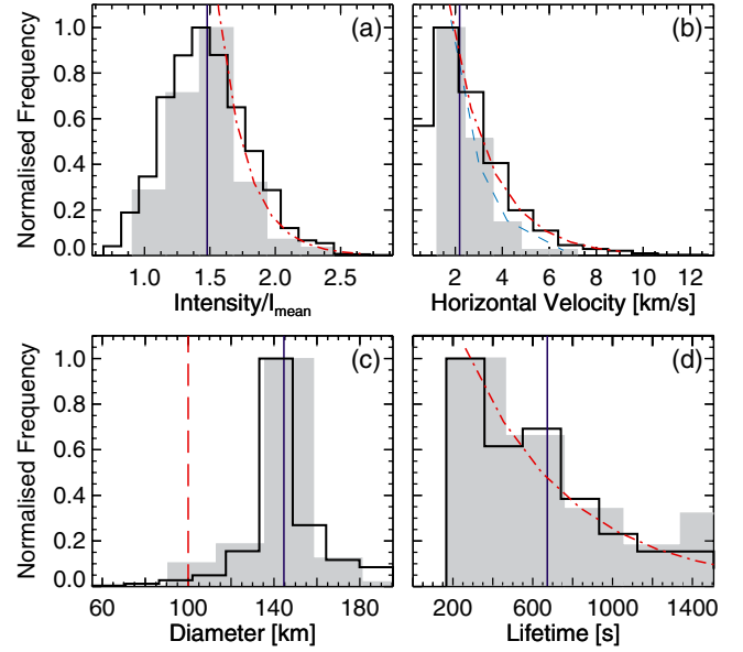
Fig. 9. Statistical properties of the detected SUNRISE Ca II H BPs. a) Distribution of mean intensity contrast for all 5677 individual measurements (black, outlined histogram) and of the time averaged contrast of all 107 BPs (grey, filled histogram). b) Distribution of all 5570 individual measurements of horizontal velocity (black, outlined histogram) and of the values averaged over their respective lifetimes of the 107 studied BPs (grey, filled histogram). c) Histogram of mean size (diameter) of all 107 BPs (grey, filled histogram) and all 5677 individual measurements (black, outlined histogram). The vertical dashed line indicates the spatial resolution achieved by the SUNRISE telescope. d) Histogram of lifetimes of 47 BPs (black, outlined histogram) and of corrected lifetimes (grey, filled histogram; see main text). The vertical solid lines indicates the mean values of the distributions. The fits (dot-dashed and dashed curves) are explained in the main text.
