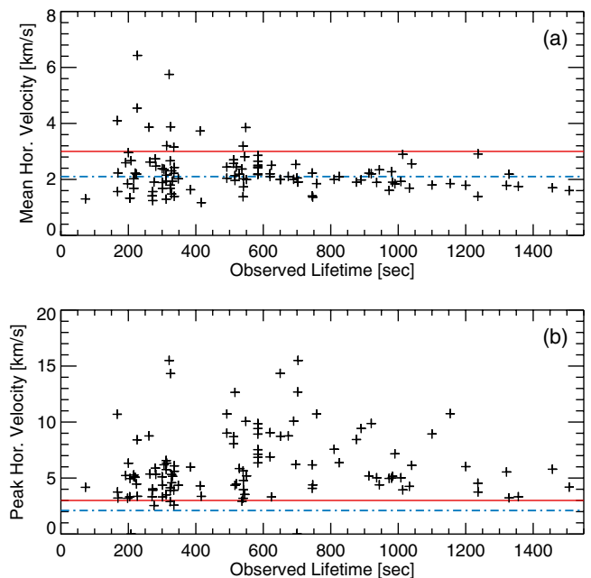
Fig. 13. a) The mean horizontal velocity, and b) maximum (peak) horizontal velocity versus the observed lifetimes of the studied BPs. The horizontal solid (red) and dot-dashed (blue) lines indicate the approximate limits for fast and intermediate BP velocities, respectively (see main text).
