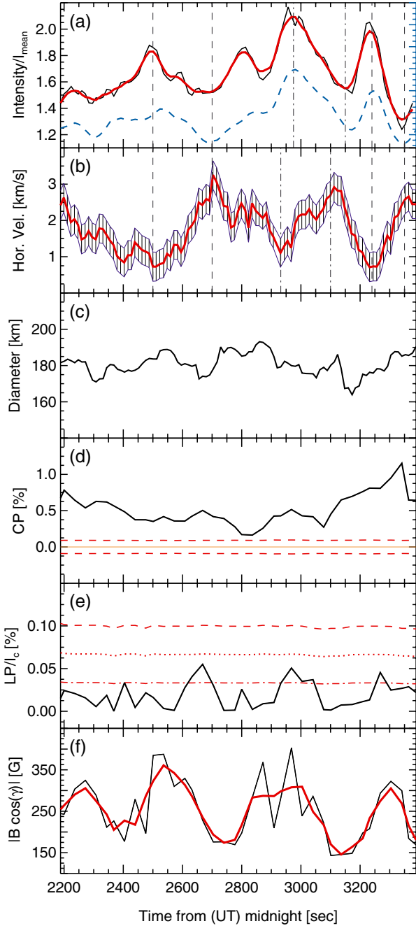
Fig. 5. Evolution of a) the intensity contrast, b) horizontal velocity, c) diameter, d) CP , a measure of the strength of Stokes V , e) total net linear polarisation LP , and f) field strength of the selected BP shown in Figs. 1 and 4. CP and LP are normalised to Stokes I continuum. In panels a) and f) , the thin curves respectively represent the time variation of average intensity and the unsigned longitudinal magnetic field within the BP while the smoothed thick lines (red in online version) show a 5-frames boxcar average. The intensities are both normalised to the mean intensity of the image. The (blue) dashed curve in panel a) represents the smoothed average intensity within the BP, in arbitrary unit, from the restored images (see main text). Evolution of horizontal velocity, smoothed within 5 frames by weighted averaging, is plotted as the thick line (red in the online version) in panel b) while the thin vertical solid lines indicate the error bars. The vertical dashed lines in the two upper panels serve to guide the eye to the general anti-correlation between intensity and horizontal velocity (see main text). The 3\sigma noise levels for both CP and LP , are drawn as dashed-lines in panels d) and e) , while the dotted and dot-dashed lines in panel e) are the 2\sigma and 1\sigma noise levels, respectively. The unsigned longitudinal magnetic field depicted in panel f) was computed from the SIR inversions (see main text).
