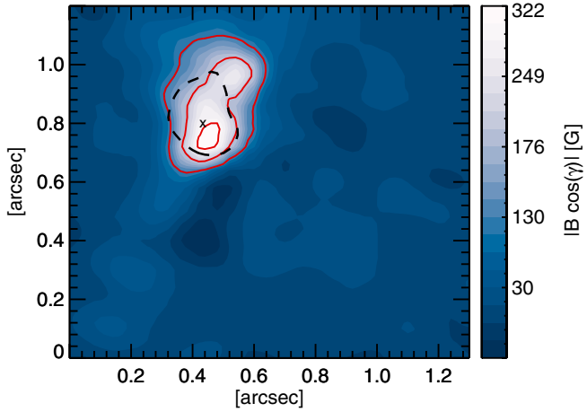
Fig. 6. Map of the unsigned longitudinal component of magnetic field, |B \cos(\gamma)| , centred on the BP shown in Fig. 4 at time 3304 s from UT midnight. The solid contours indicate the height-independent |B \cos(\gamma)| at 100, 200 and 300 G. The Ca II H BP's area is indicated by the dashed contour.
