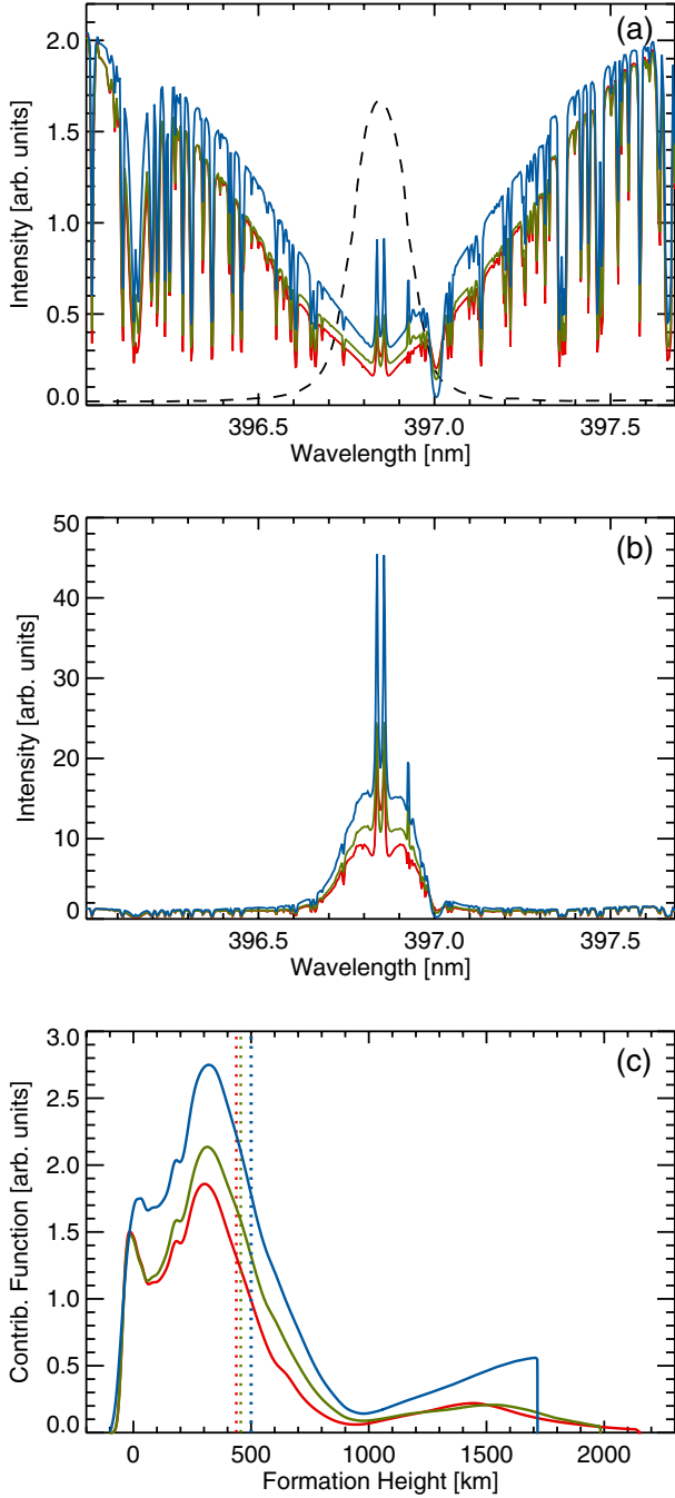
Fig. 2. a) Intensity profiles (synthetic spectra) of Ca II H line for three atmospheric models (see text). The dashed curve represents the transmission profile of the SUNRISE/SuFI Ca II H filter. b) Results of the convolution of the spectra with the transmission profile shown in panel a). c) Line depression contribution functions for the SUNRISE/SuFI Ca II H bandpass vs. height. The vertical lines indicate the corresponding average heights formation. Red, green and blue lines in all panels represent the FALC, FALF and FALP model atmospheres.
