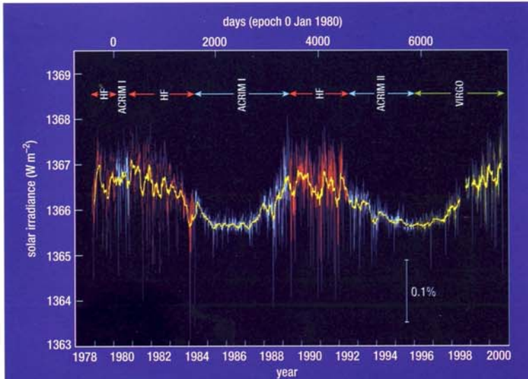
6: Composite of total solar irradiance covering more than two solar cycles, as measured by radiometers flying on spacecraft. Data from four instruments have been used to create this composite. Details of the procedure employed to merge the data sets are provided by Fröhlich and Lean (1998).
