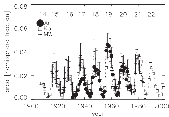
Fig. 9. Temporal variation of yearly median values of the plage coverage measured from the Arcetri, Kodaikanal, and Mt. Wilson series. The error bars represent the standard deviation of measured values over the annual interval; for clarity, they are only shown for the MW series. Cycle numbers are given at the top of each cycle. From Ermolli et al. (2009).
