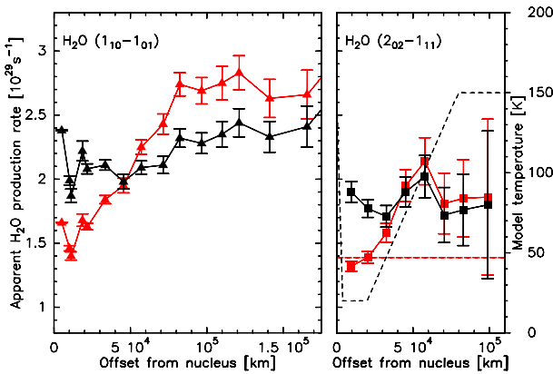
Fig. 3. Apparent H 2 O production rates as a function of beam offset deduced from the 557 GHz ( left ) and 988 GHz ( right ) H 2 O maps observed on 6.56 and 6.60 October UT, respectively. Calculations with a 47 K and variable T_{\text{kin}} are shown with red and black symbols, respectively. The temperature profiles are plotted in the right panel with dashed lines.
