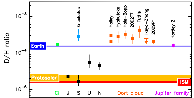
Fig. 4. D/H ratio in the water of comets (including the revised value for Halley from Brown et al. 2012) compared to values in carbonaceous meteorites (CI), the Earth's oceans, and Enceladus. Displayed data for planets, interstellar medium (ISM), and the protosolar nebula refer to the value in \text{H}_2 . Adapted from Hartogh et al. (2011).
