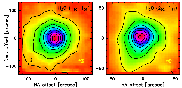
Fig. 2. On-the-fly maps of \text{H}_2\text{O} in C/2009 P1 (Garradd) obtained with the WBS. Left: the 1_{10}-1_{01} 557 GHz line observed on 6.291 October 2011 UT. Right: the 2_{02}-1_{11} line at 988 GHz observed on 6.597 October 2011 UT. The contour spacing is 1 \text{K km s}^{-1} in brightness temperature, corresponding to \sim 6\sigma . The Sun direction is indicated at lower right. The beam sizes are 38''.1 and 21''.5 at 557 GHz and 988 GHz, respectively.
