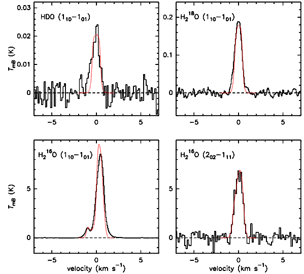
Fig. 1. HIFI spectra of comet C/2009 P1 (Garradd) observed on 6 October 2011 with the HRS. HDO (509 GHz), \text{H}_2\text{O} (557 GHz), and \text{H}_2^{18}\text{O} (548 GHz) 1_{10}-1_{01} spectra are the average of single-point measurements. The spectrum of the \text{H}_2\text{O} 2_{02}-1_{11} line at 988 GHz is extracted from the map, by averaging data at offsets <10'' from the peak. The velocity scale is given with respect to the comet rest frame. Synthetic line profiles obtained with 30% extended production (see text) are shown by red dotted lines. Gas acceleration (velocity increasing from 0.48 \text{km s}^{-1} to 0.58 \text{km s}^{-1} from r = 10^4 km to 10^5 km) is considered to fit more closely the wings of the profiles (Combi et al. 2004).
