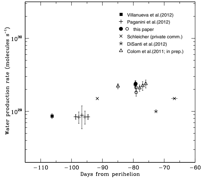
Fig. B.1. Water production rates measured pre-perihelion in comet C/2009 P1 (Garradd). The time is with respect to the perihelion (23 December 2011). The plain and empty circles correspond to the 6-October single-point and mapping HIFI observations, respectively, analysed with the model with T_{\text{law}} .
