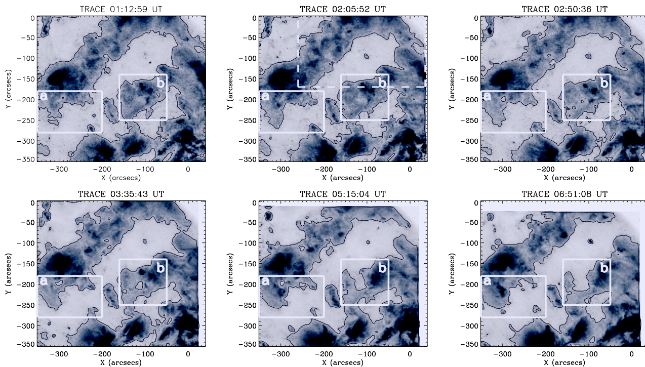
Fig. 5. Reversed color TRACE 171 Å images showing a partial field-of-view of CH2 observed in November 1999. The over-plotted rectangular areas (a and b) are shown enlarged in Figs. 6 and 7. The dashed line box corresponds to the field-of-view presented in Fig. 8.
