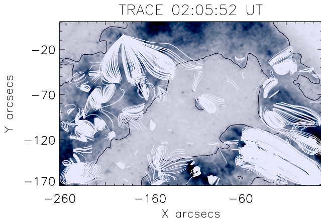
Fig. 8. TRACE 171 Å image with a field-of-view as shown in Fig. 5 with over-plotted only closed magnetic field lines connecting magnetic polarities above 20 G. The magnetic field lines were obtained with a potential magnetic field extrapolation (Wiegmann et al. 2005).
