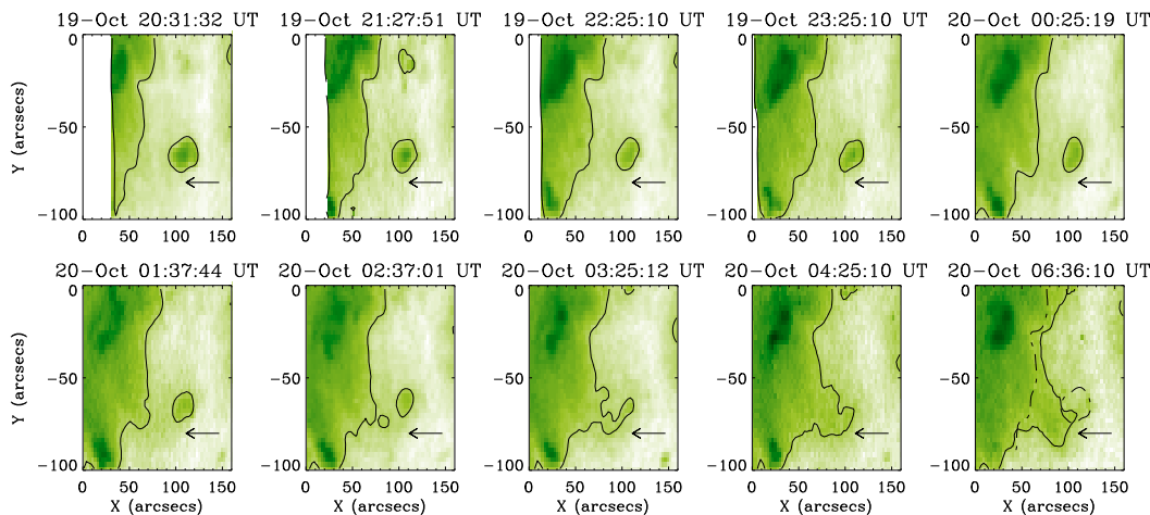
Fig. 4. EIT images of the area marked with “b” in Fig. 2 (reversed color table). The arrows point to a bright point whose evolution led to the contraction of the coronal hole. The over-plotted dashed-dotted line shows the boundary from the first image.
