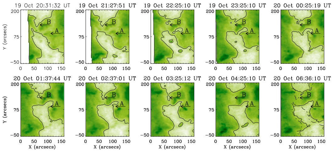
Fig. 3. EIT images of the area marked with “a” in Fig. 2 (reversed color table). The arrows point to the BPs whose evolution led to the expansion (arrow A) and the contraction (arrow B) of the CH. The over-plotted dashed-dotted line shows the boundary from the first image.
