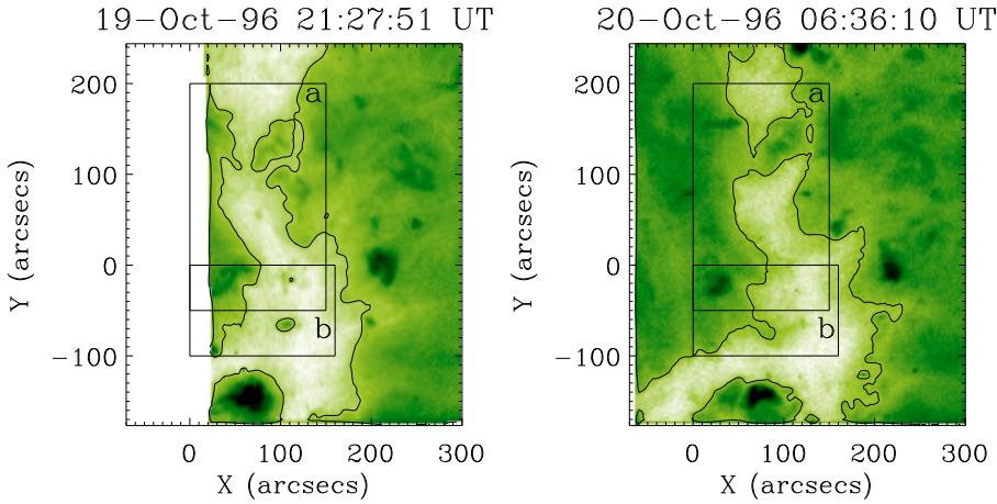
Fig. 2. Color table reversed EIT 195 Å images of the coronal hole observed on October 19–20, 1996. The over-plotted rectangular areas (a) and b) are shown enlarged in Figs. 3 and 4.
