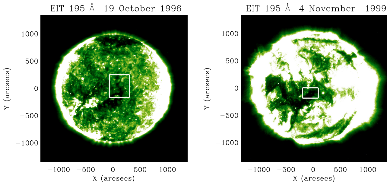
Fig. 1. Full-disk EIT 195 Å images obtained on 1996 October 19 and 1999 November 4. The over-plotted boxes outline the field-of-views subjected to detailed study.
